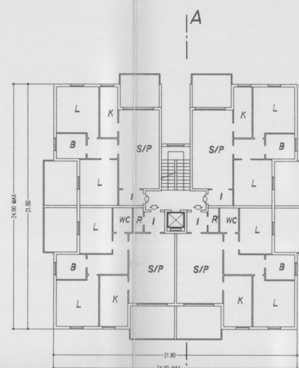
PIANO 1-2-3-4
