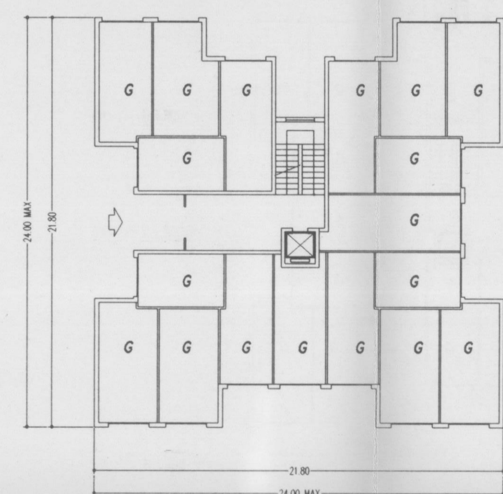
PIANO TERRA
