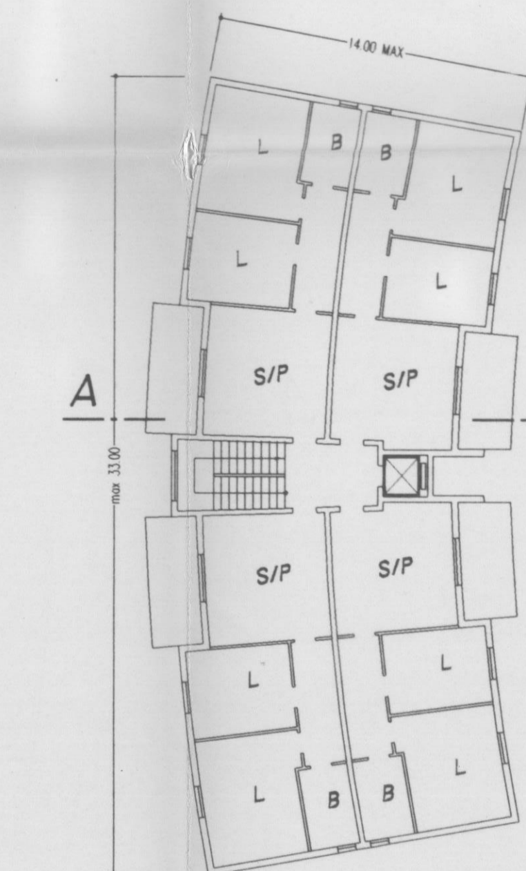
PIANO 1-2-3-4-5
