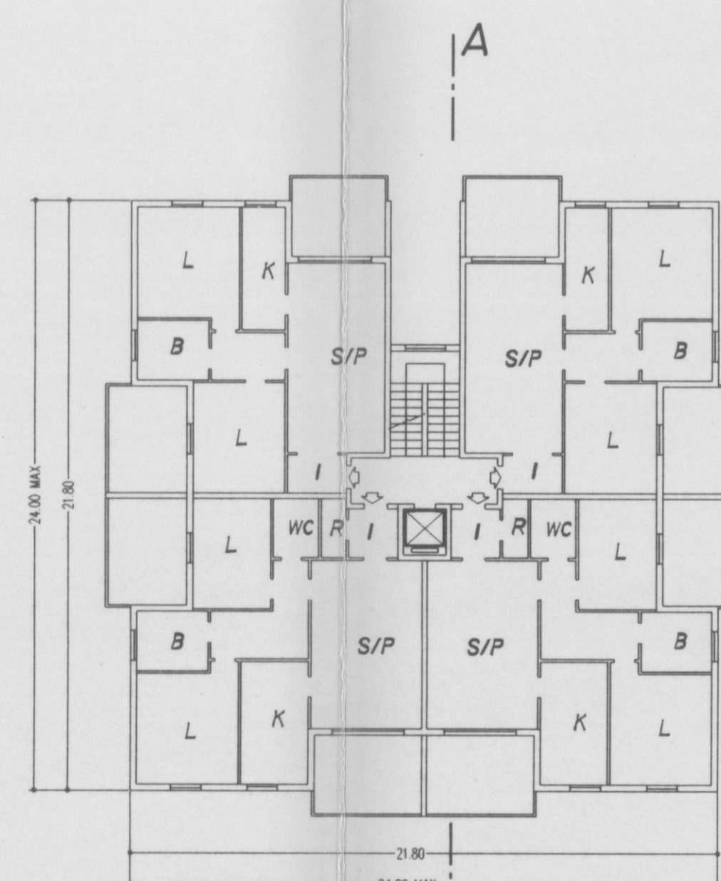
PIANO 1-2
